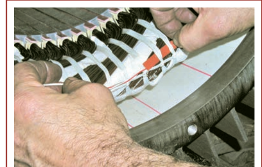
Sensor with silicone rubber body pictured above inserted near EndTurn of windings.
